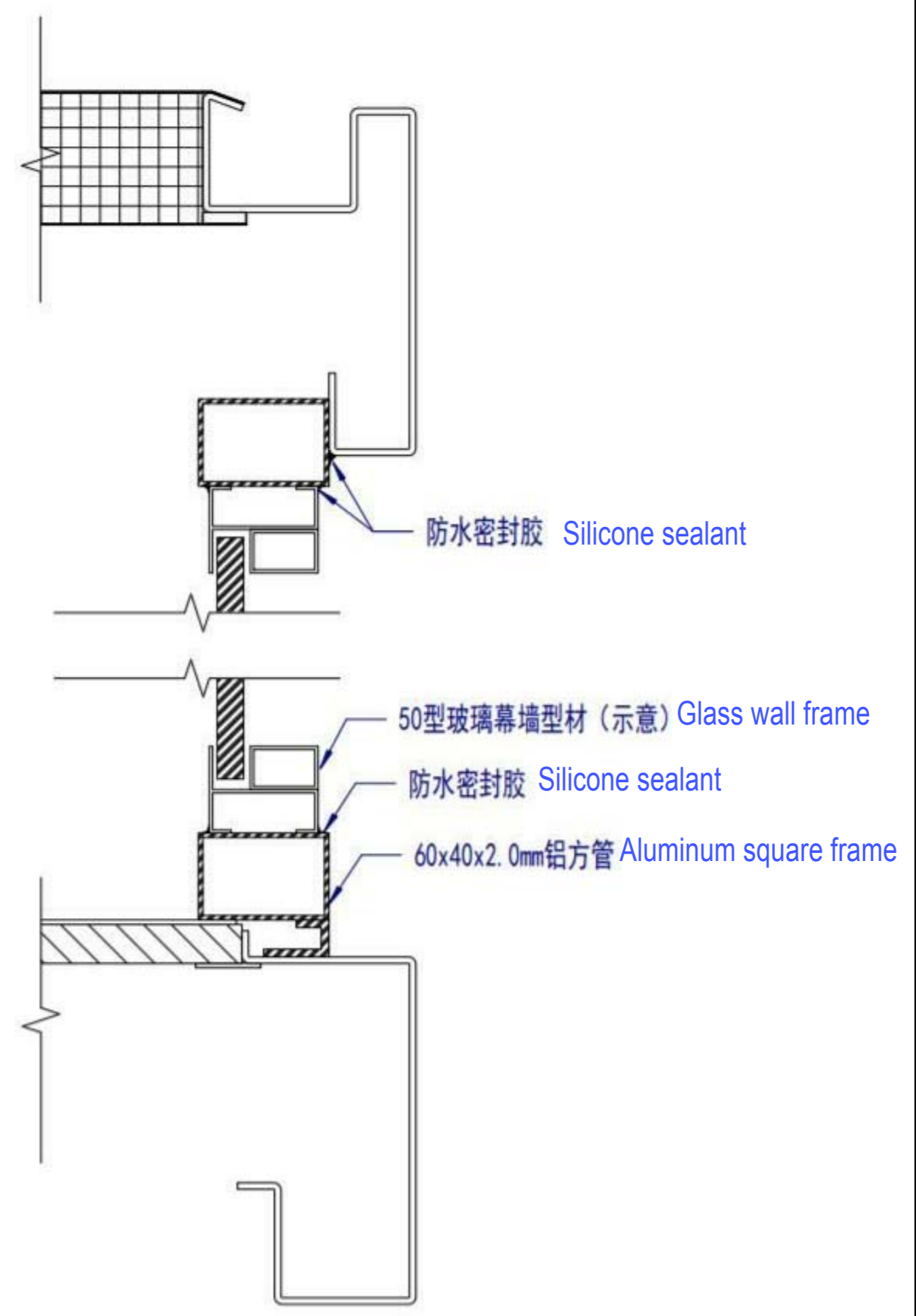
Glass Wall Section
