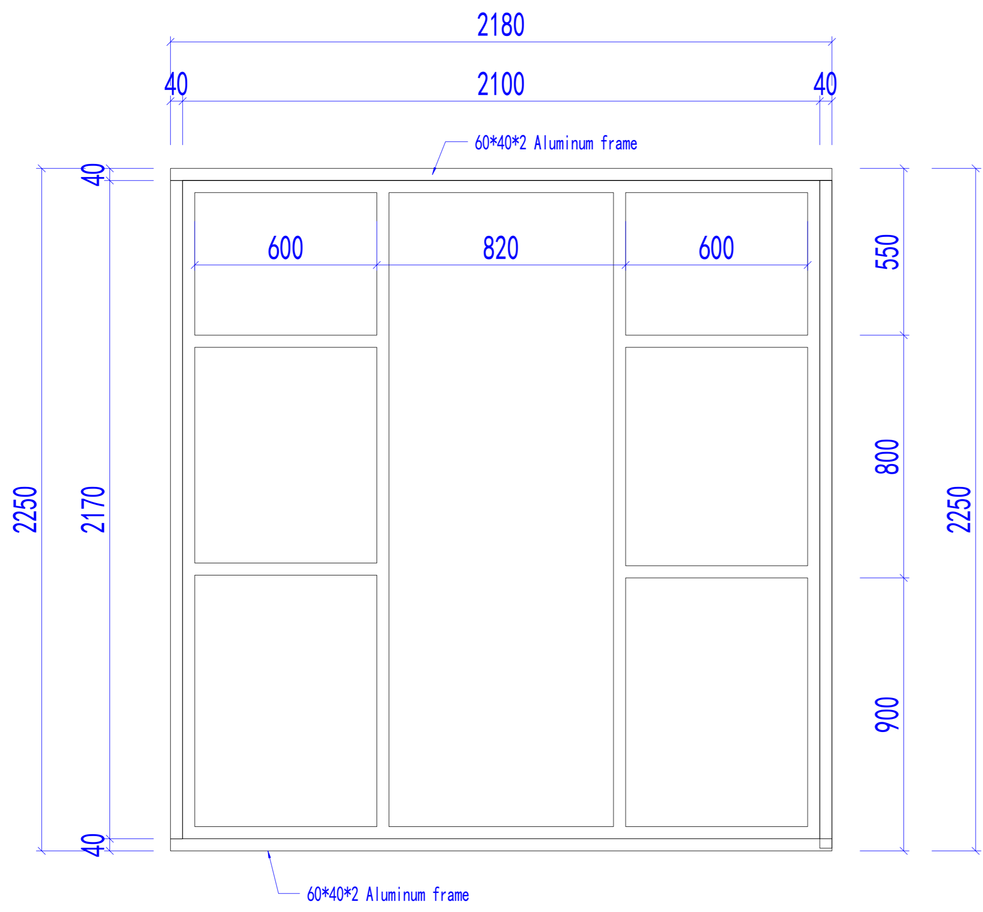
W2 Glass Wall Detail
