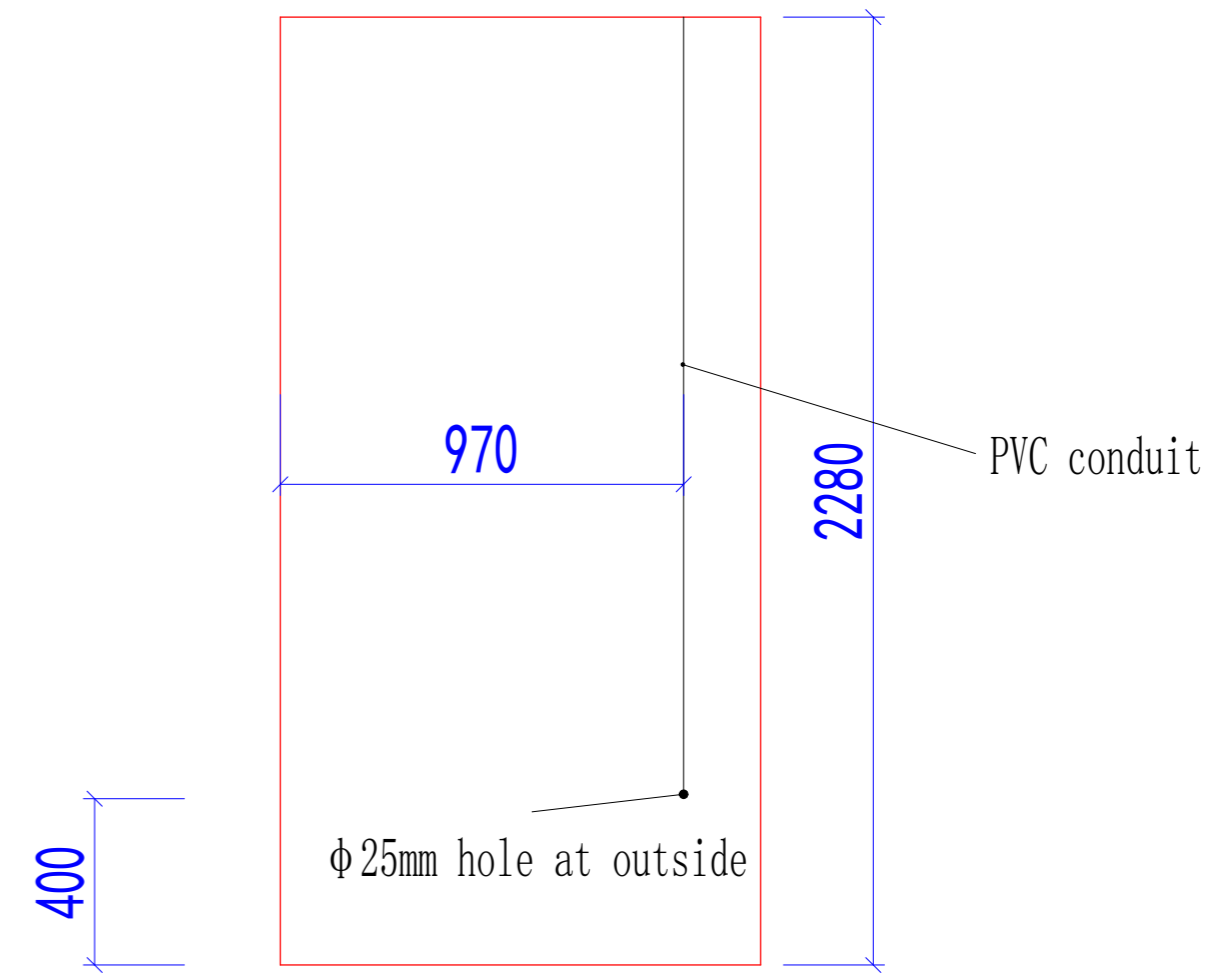
Wall Panel Detail
